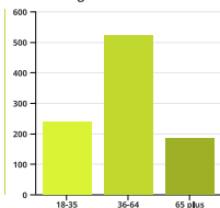
Age Distribution
